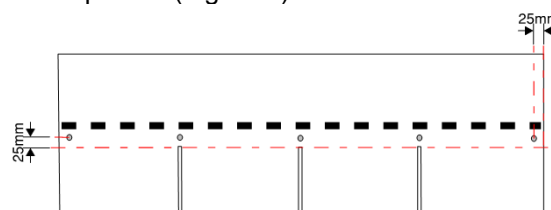
Figure 2 - Installing the shingle
